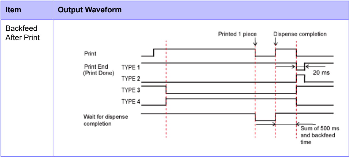
Timing Chart of the Wait Signal for Dispense Completion
