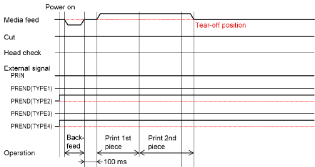
Timing Chart (When <TW> is 500)
